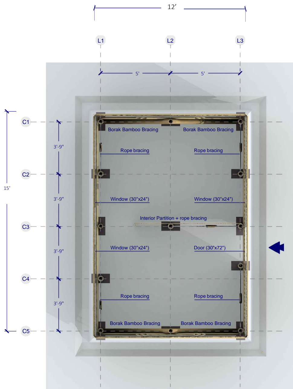
Borak Bamboo Bracing
